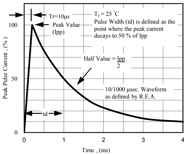
Fig. 3 - Pulse Waveform
